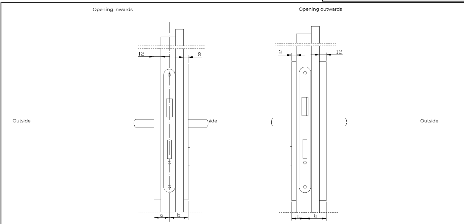
Above drawing applies to "Porta Agat", "Porta Agat Plus", "Porta Opal", "Porta Opal Plus", "Porta Granit", "Porta Granit Plus" and "Porta Safe".
